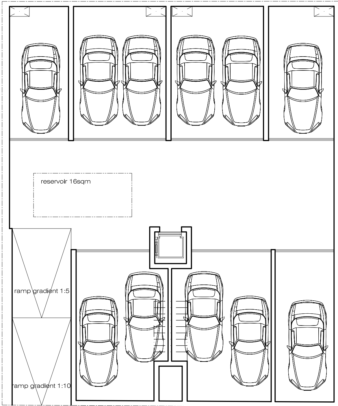
PROPOSED semibasement floor plan — Scale 1:100 —
